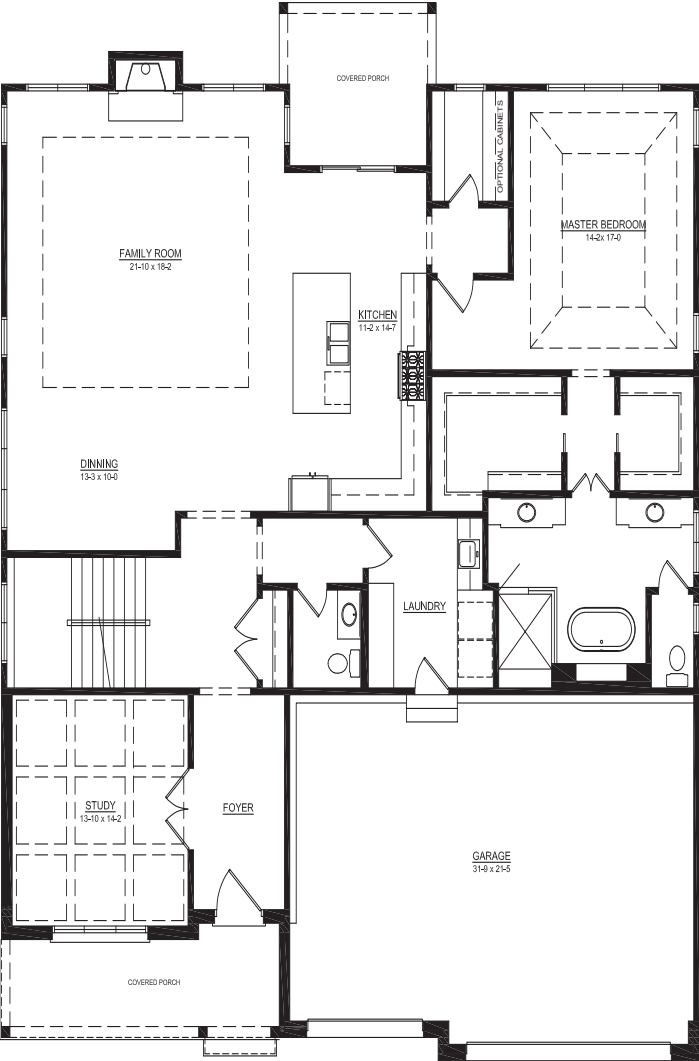
FIRST LEVEL FLOOR PLAN
