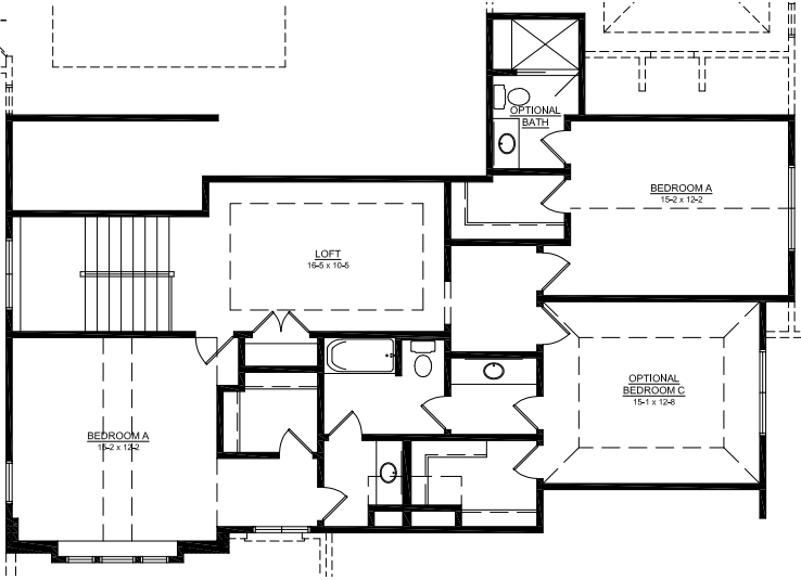
OPTIONAL SECOND FLOOR PLAN 300 sq. ft.
