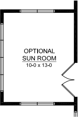
OPTIONAL FIRST FLOOR PLAN - SUNROOM 150 sq. ft.
