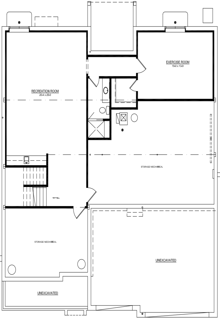
OPTIONAL LOWER LEVEL FLOOR PLAN 1,250 sq. ft.
