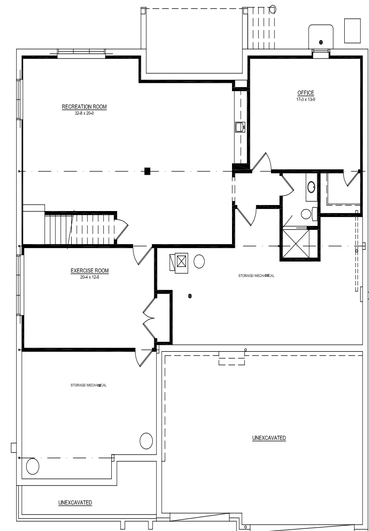
OPTIONAL LOWER LEVEL FLOOR PLAN 1,450 sq. ft.
