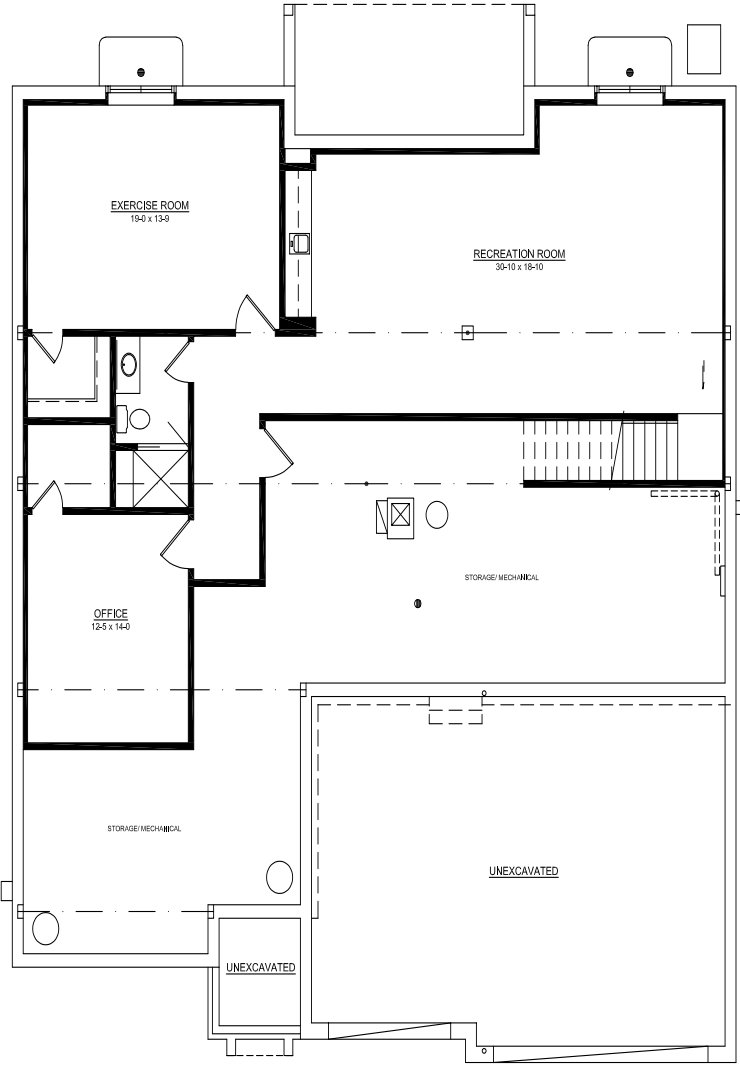
OPTIONAL LOWER LEVEL FLOOR PLAN 1,350 sq. ft.
